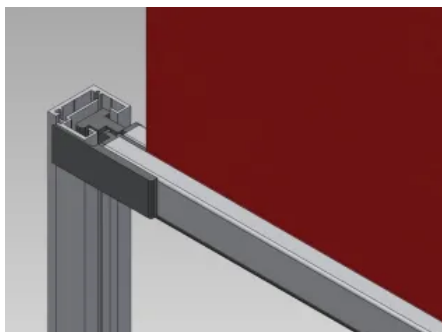
C-Schiene BS-C-MQ1
