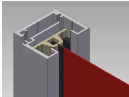
ZIP-Schiene BS-ZIP-MQ
