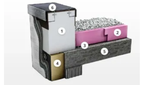
Austrotherm Attikaelement
