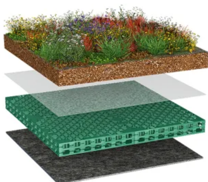
BauderGREEN Retention System Drossel
