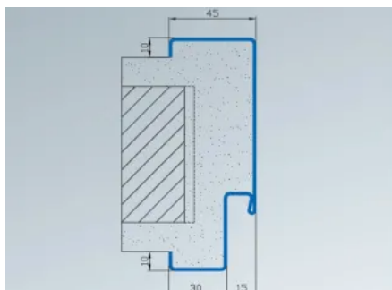
Gipswandzarge Profil 23/0045 | Drahtanker
