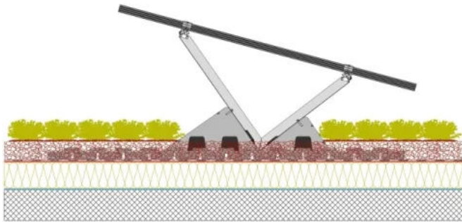
Contec.greenlight - Systemskizze
