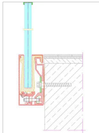
GM RAILING® UNI SIDE
