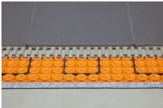
Schlüter®-DITRA-HEAT-DUO-PS
