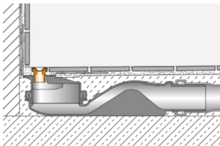
Schlüter®-KERDI-LINE-VARIO COVE
