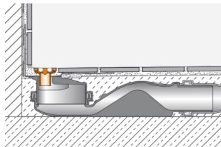
Schlüter®-KERDI-LINE-VARIO WAVE
