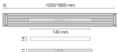
KERDI-LINE-VARIO WAVE 34
