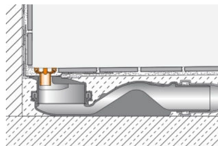
Schlüter®-KERDI-LINE-VARIO WAVE
