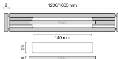
KERDI-LINE-VARIO WAVE 42 Alu
