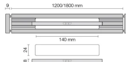
KERDI-LINE-VARIO WAVE 42 Alu
