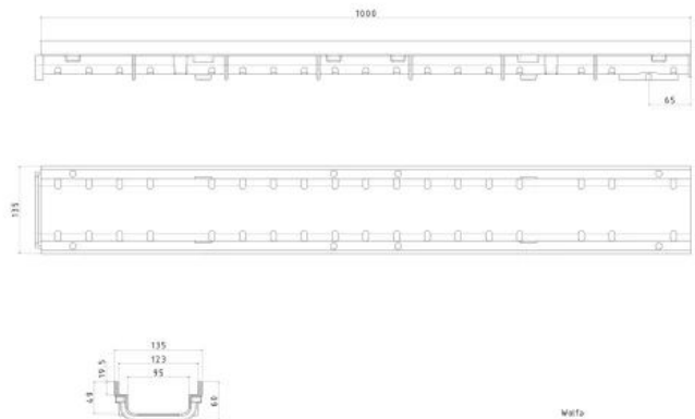
WOLFA Rinne 100/6V Drain
