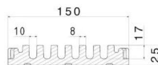
AquaStop 150-OS*, 150 x 25 mm
