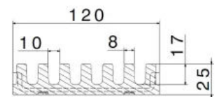
AquaStop Ultra 120-10, 120 x 25 mm
