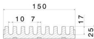
AquaStop Ultra 150, 150 x 25 mm
