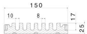
AquaStop 150-OS*, 150 x 25 mm
