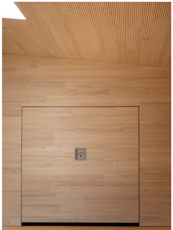
StudioLine Solo
