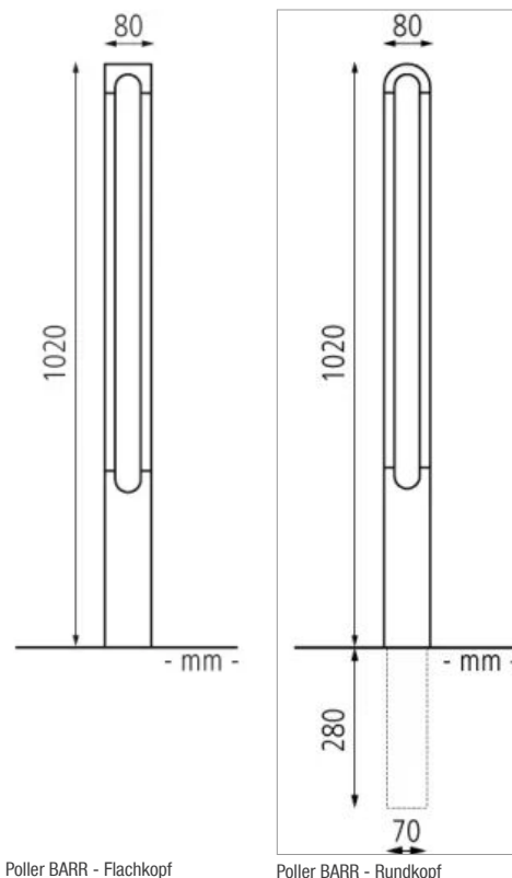
Poller BARR - Flachkopf
