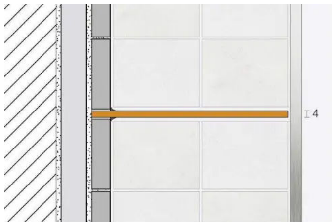
Schlüter®-SHELF-N
