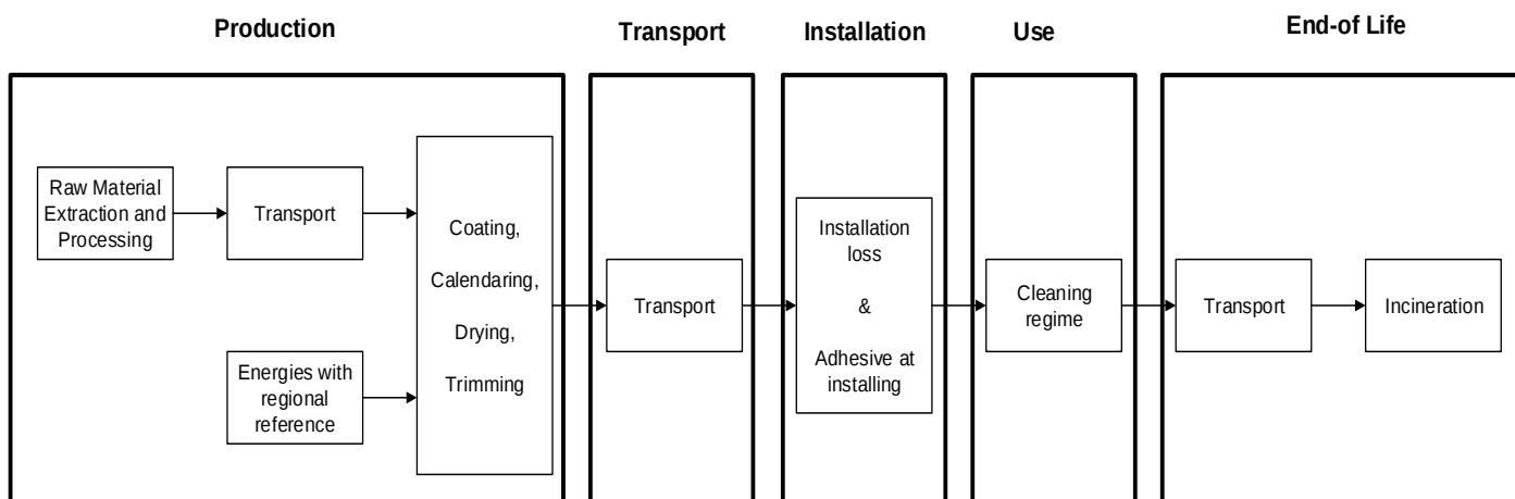
Figure 3: Flow chart of the Life Cycle Assessment
