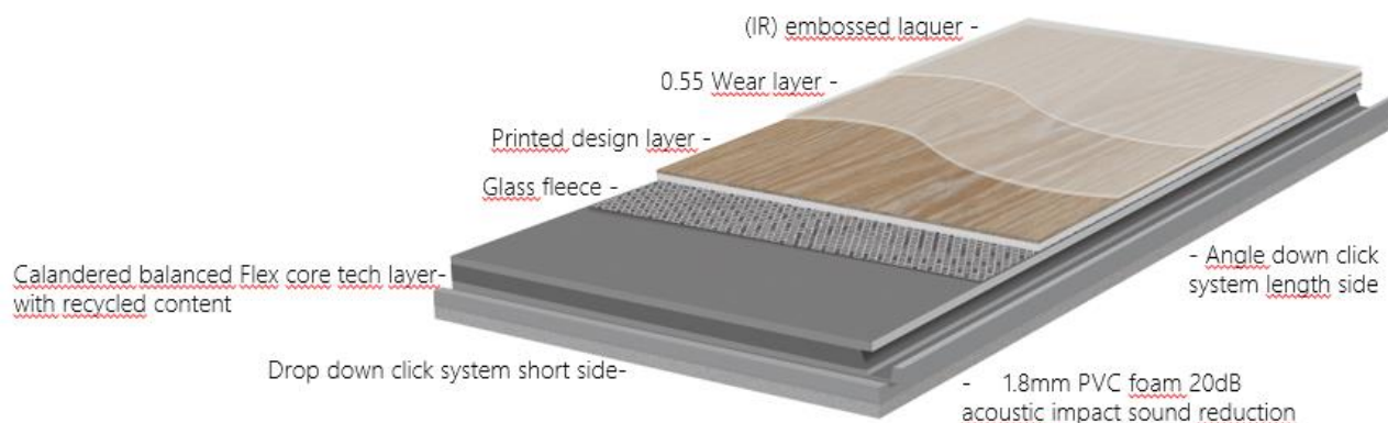
Figure 1: Typical construction Allura click Flexcore
