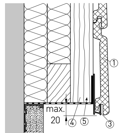
Ⓓ Montagebeginn, Alternative
