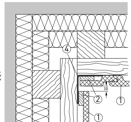
Ⓓ Innenecke, Alternative
