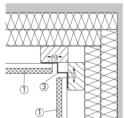
Ⓕ Innenecke, Alternative
