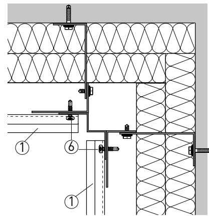
(C) Alu- Innenecke
