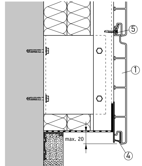
(C) Montagebeginn
