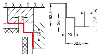
Alu-Inneneckprofil
