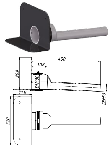
Attikaablauf FPO-PP DN 50
