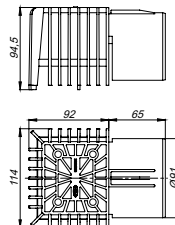
Attika-Laubfangkorb
