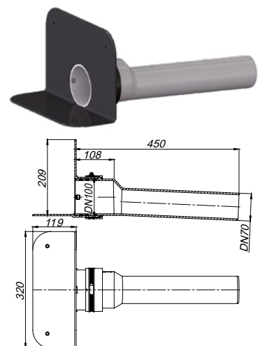
Attikaablauf FPO-PP DN 70
