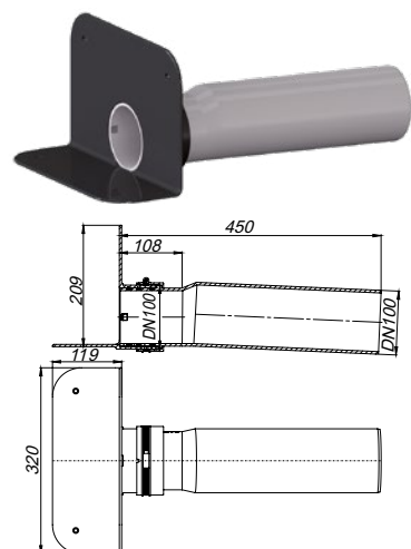
Attikaablauf FPO-PP DN 100
