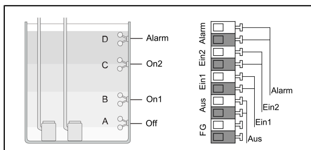
Fig. 2: Float switches Duo
