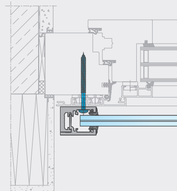
Holz-Aluminium-Fenster
