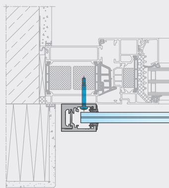
Aluminium-Fenster
