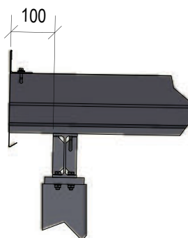
Detail B
