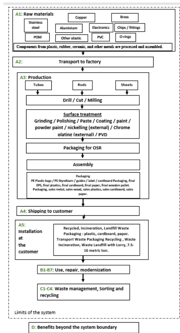
Figure 3: Flow diagram of product system with modules A1-D
