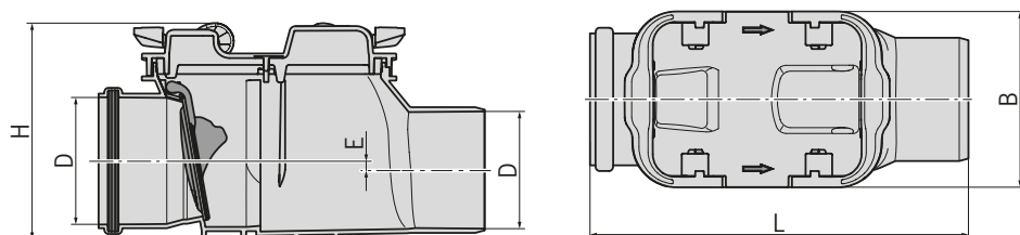
Figure: Single backflow stop (type 0)
