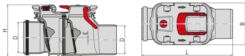
Figure: Double backflow stop (type 2)
