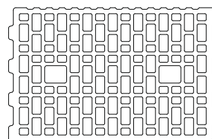
Lochbild 5) T0,8-240 EB
