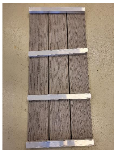
Figure 2: Picture of the received sample (back)
