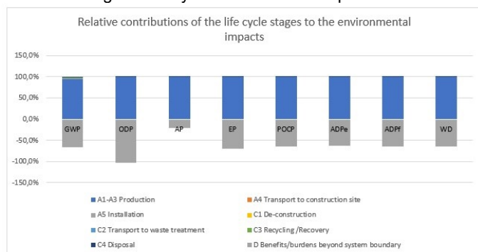
Figure 1: Relative environmental impacts of the different life cycle stages for the VELUX interior roller blind DKL (Modules A1-C4 = 100%)
