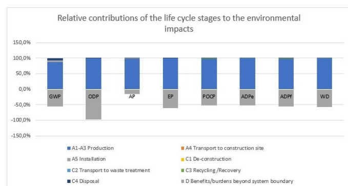
Figure 1: Relative environmental impacts of the different life cycle stages for the VELUX interior roller blind DKY - Nature Collection (Modules A1-C4 = 100%)
