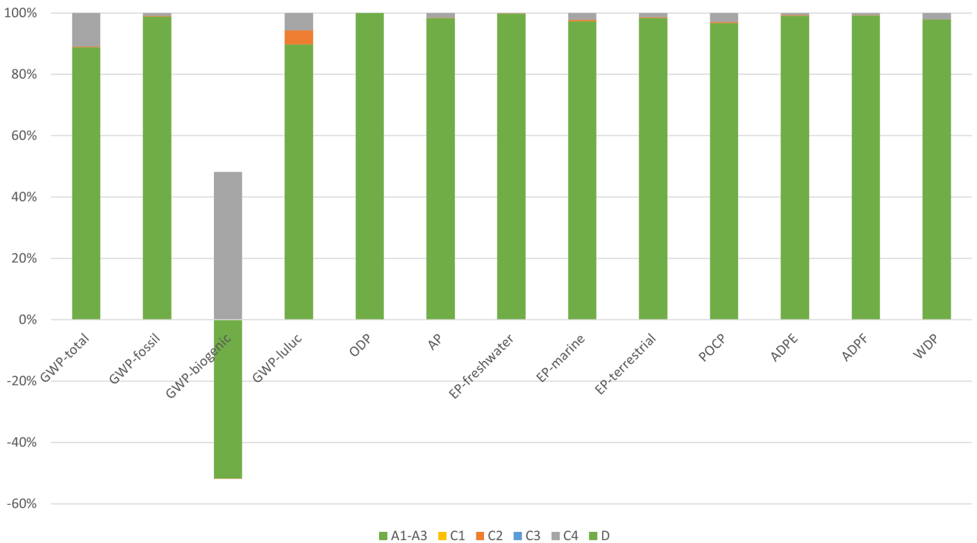
Hot-spot analysis of ZENTIA wet felt laminated mineral ceiling tiles
